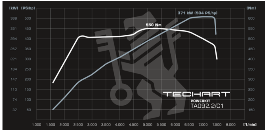
Image 8: Performance chart TECHART TECHTRONIC Powerkit for 911 (992.2) Carrera
