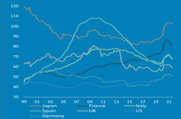
Figure 12: Non-Financial Corporations (NFC) debt ratio, in % of GDP, selected countries
