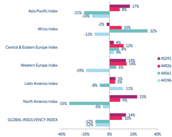
Figure 16: Global and regional insolvency indices, yearly change in %
