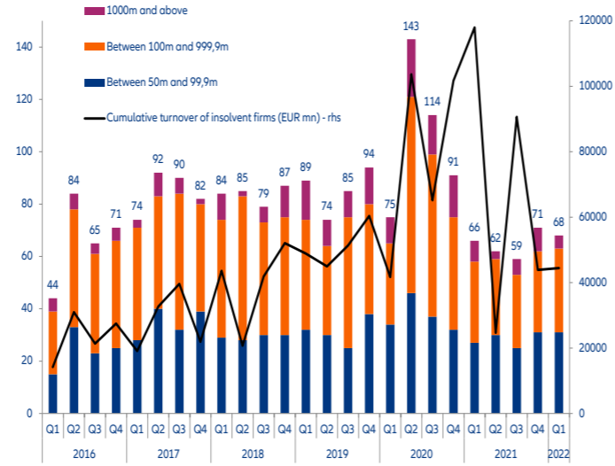
Figure 11: Major insolvencies, quarterly number by size of turnover in EURmn
