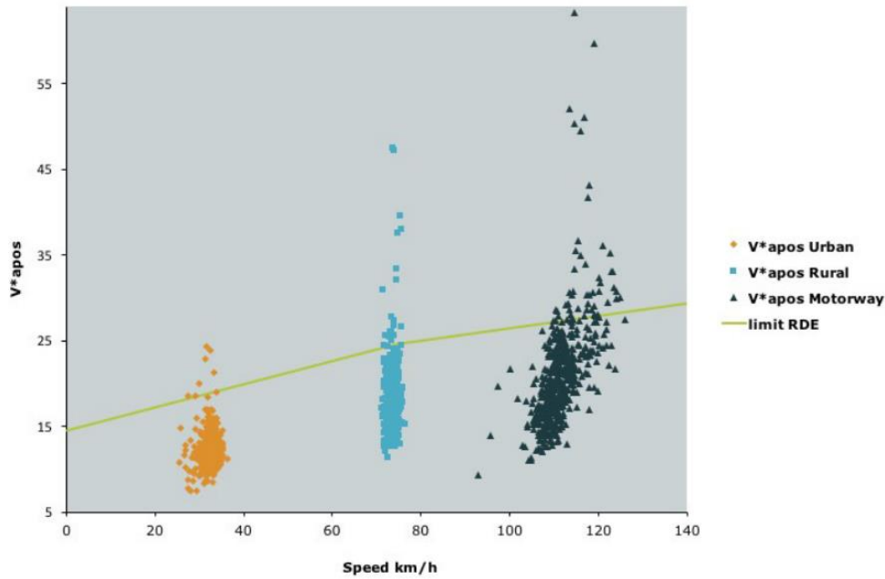
Figure 5 - Comparison of the driving conditions of 340 on-road tests done on PSA vehicles with the EU RDE upper limit
