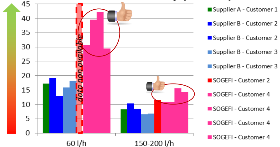
Heater Efficiency (°K/kW)
